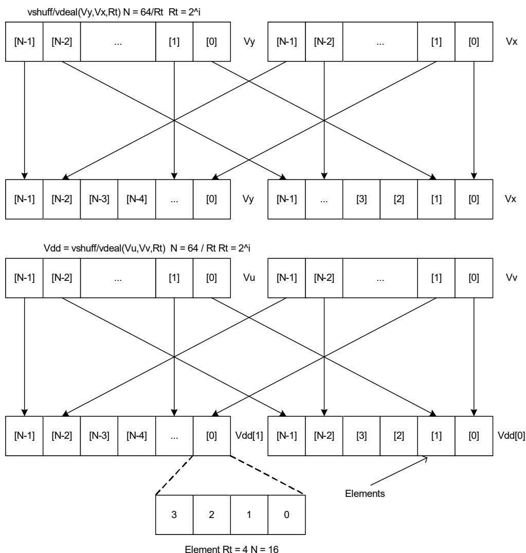
Figure 6-4 vshuff/vdeal (Vy,Vx, Rt) N = 64/Rt Rt = 2 i
