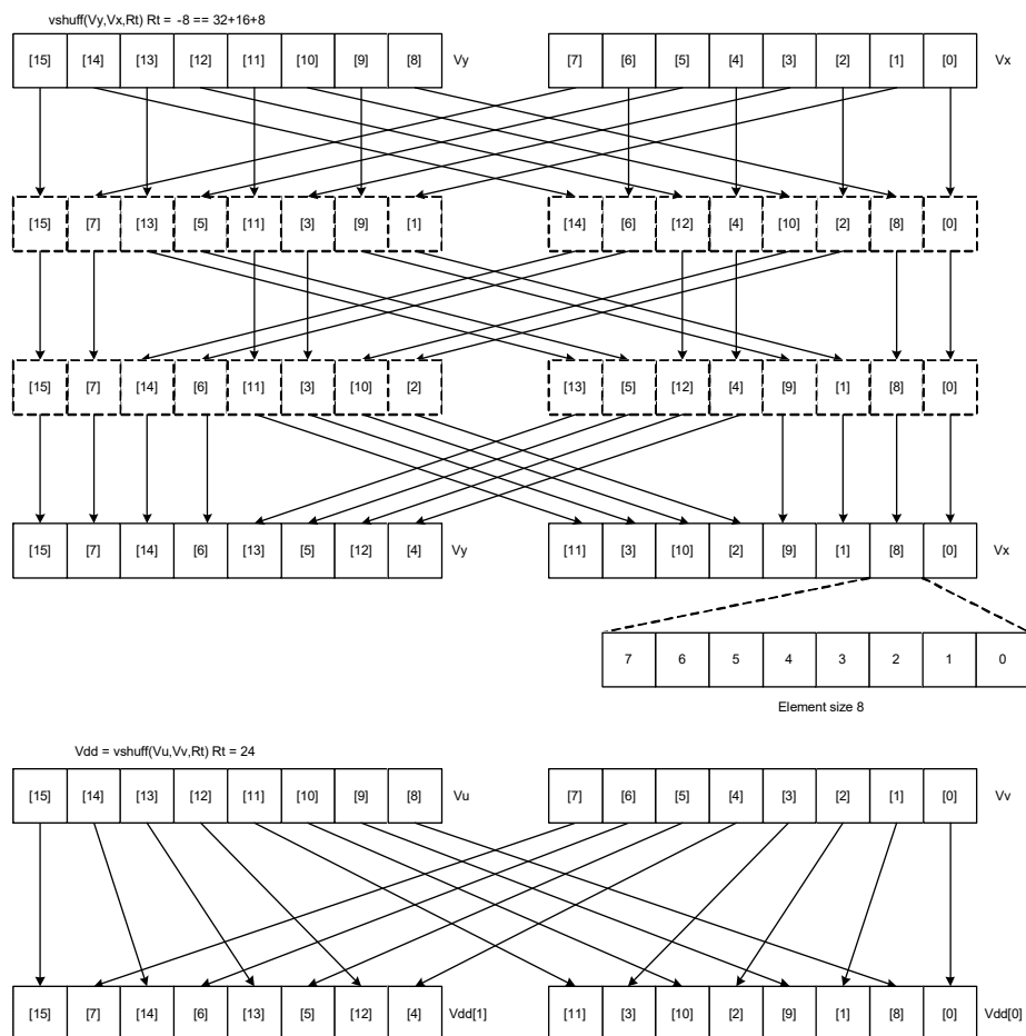
Figure 6-5 vshuff(Vy, Vx, Rt) Rt = -8 == 32 + 16 + 8
