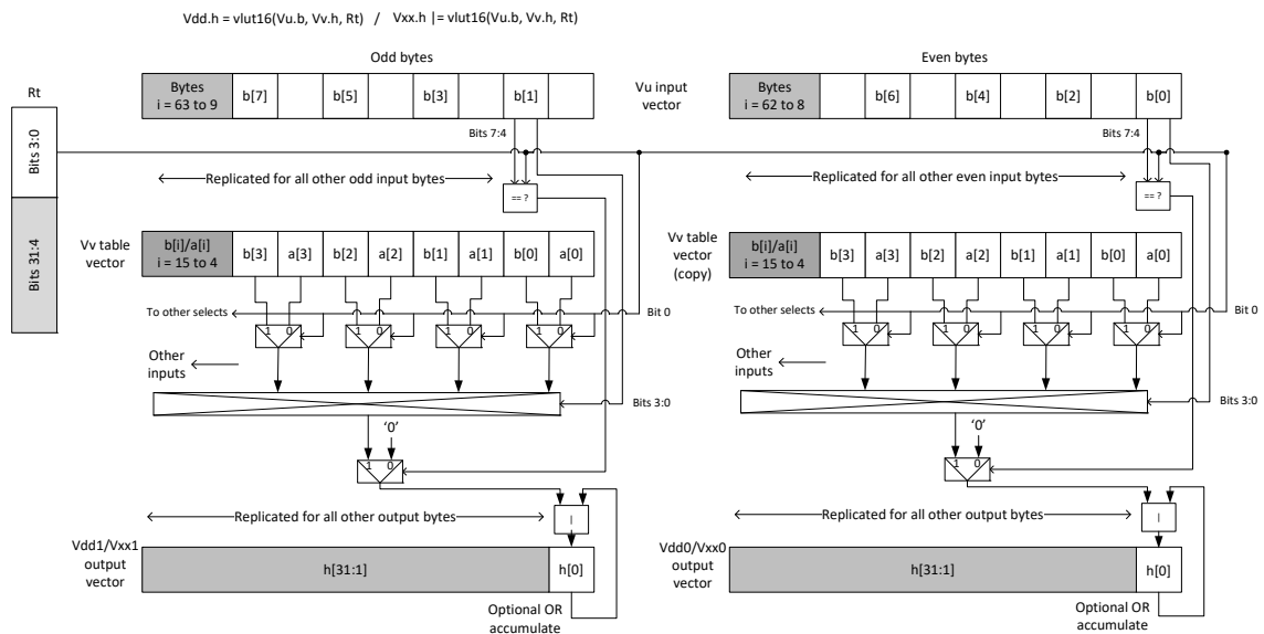
Figure 6-3 Vlut16 with even bytes used to look up a table value
